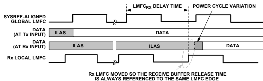
Figure 115. Adjusting the JESD204B Rx LMFC in the Logic Device
