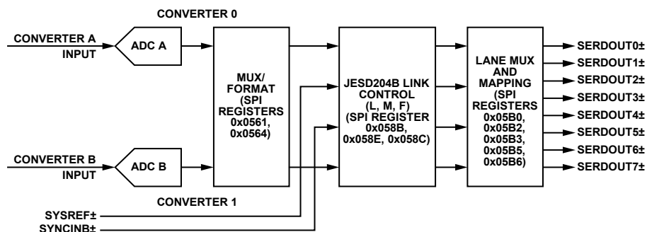
Figure 101. Transmit Link Simplified Block Diagram Showing Full Bandwidth Mode (Register 0x0200 = 0x00)
