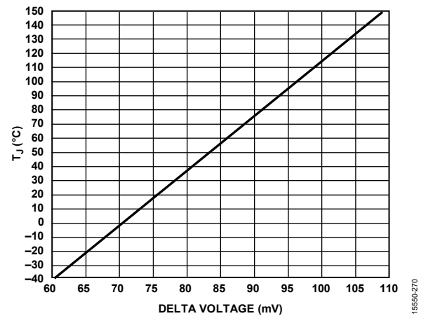
Figure 70. Junction Temperature vs. \Delta V (mV)
