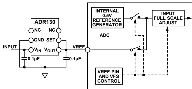
Figure 56. External Reference Using the ADR130
