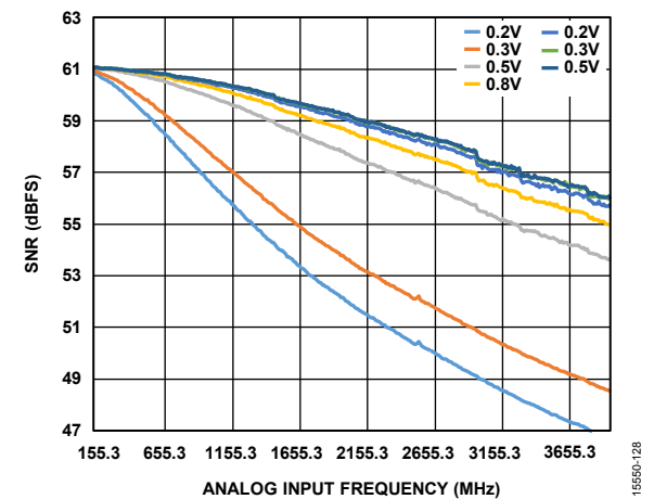
Figure 28. SNR vs. Analog Input Frequency ( f_{IN} ) vs. Various Clock Amplitude in Differential Peak-to-Peak Voltages
