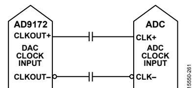
Figure 61. DAC Clock Output Clocking the AD9689
