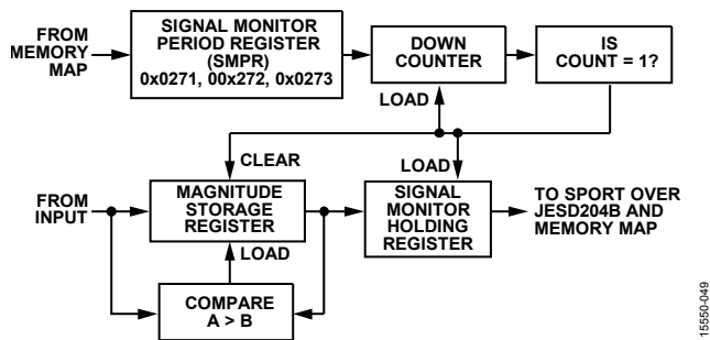
Figure 97. Signal Monitor Block
