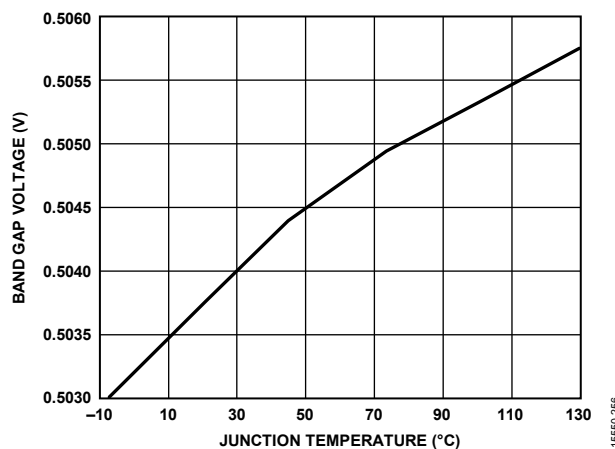
Figure 54. Typical Reference Voltage ( V_{REF} ) Drift
