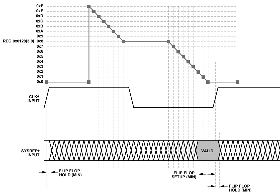
Figure 124. SYSREF± Setup Detector
