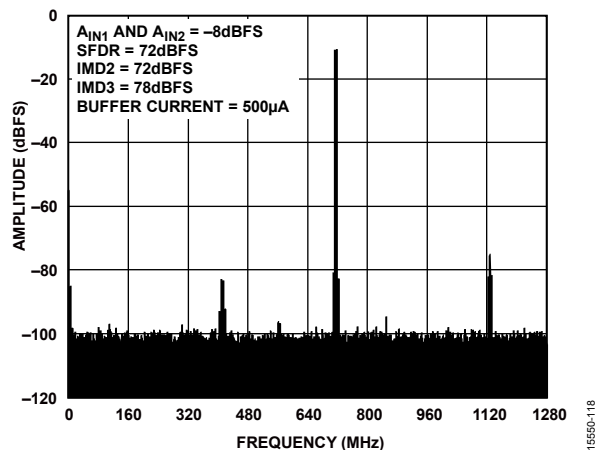
Figure 18. Two-Tone FFT; f_{IN1} = 1841 MHz, f_{IN2} = 1846 MHz; A_{IN1} and A_{IN2} = -8 dBFS
