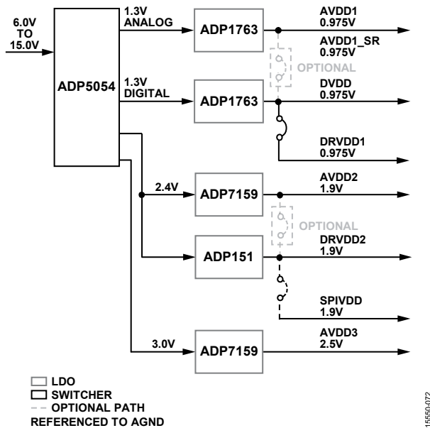
Figure 127. High Efficiency, Low Noise Power Solution for the AD9689
