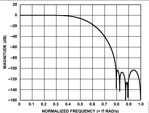
Figure 91. HB2 Filter Response
