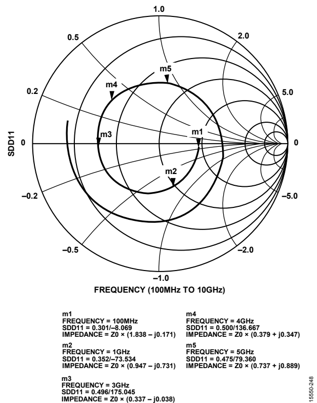
Figure 48. Differential Input Return Loss
