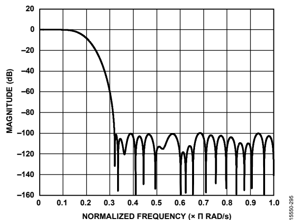
Figure 95. FB2 Filter Response
