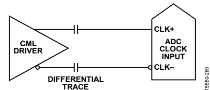
Figure 60. Differential CML Sample Clock
