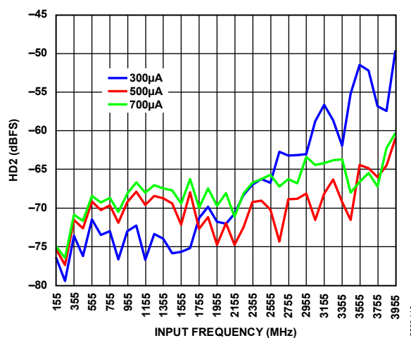
Figure 16. Second Harmonics ( HD2 ) vs. Input Frequency ( f_{IN} ) for Various Buffer Currents
