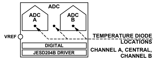
Figure 67. Temperature Diode Locations in the Die
