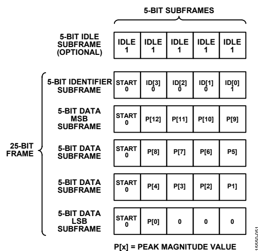
Figure 99. SPORT over JESD204B Signal Monitor Frame Data
