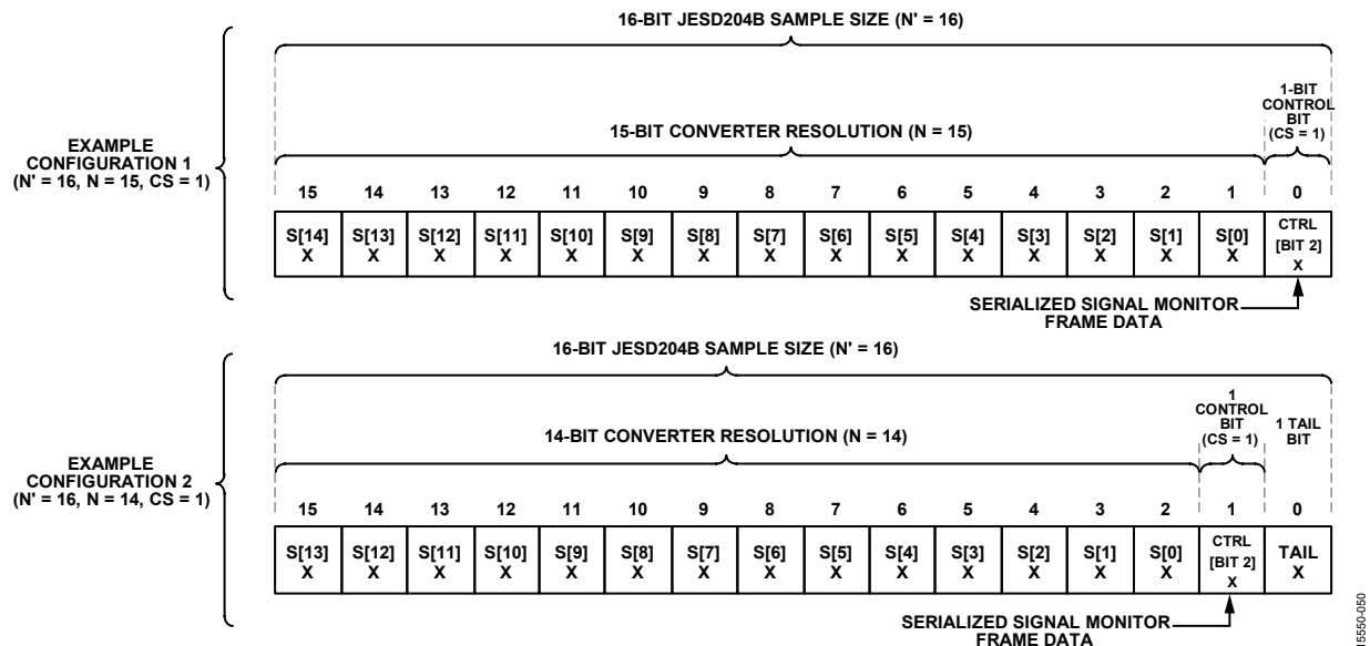
Figure 98. Signal Monitor Control Bit Locations
