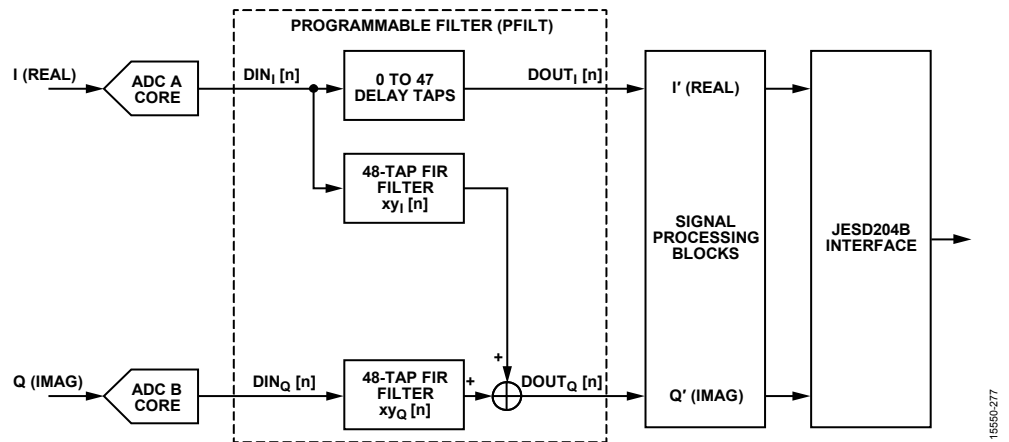
Figure 77. 48-Tap Half Complex Filter Configuration
