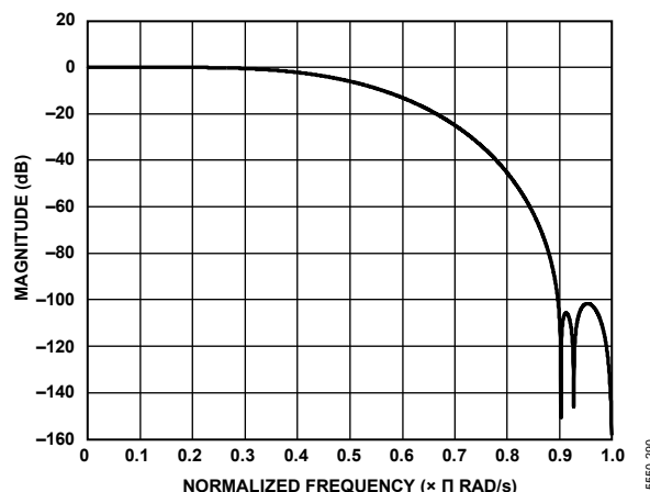
Figure 90. HB3 Filter Response
