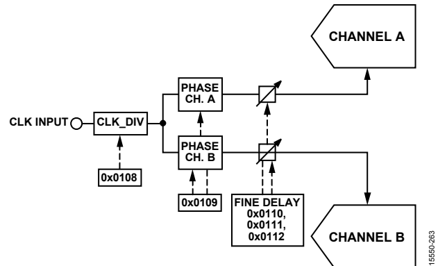
Figure 63. Clock Divider Phase and Delay Controls
