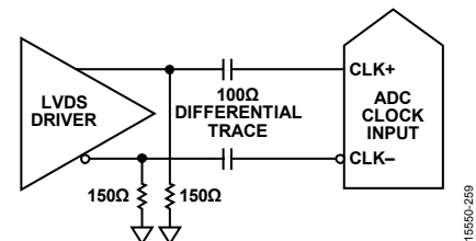
Figure 59. Differential LVPECL Sample Clock
