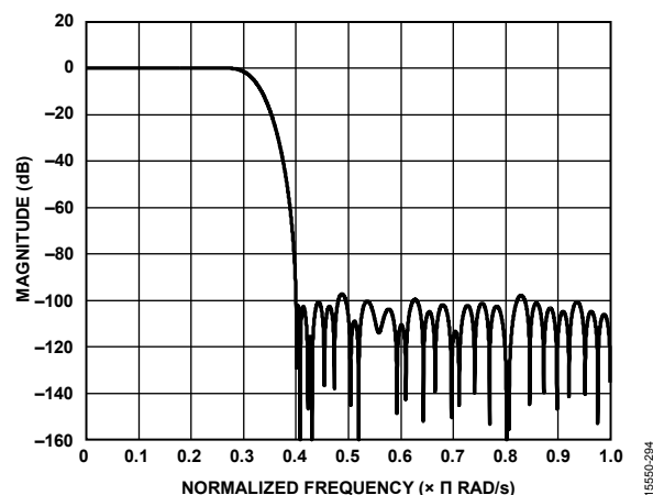
Figure 94. TB1 Filter Response
