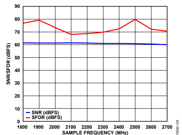
Figure 29. SNR/SFDR vs. Sample Frequency ( f_s ), f_{IN} = 900 MHz
