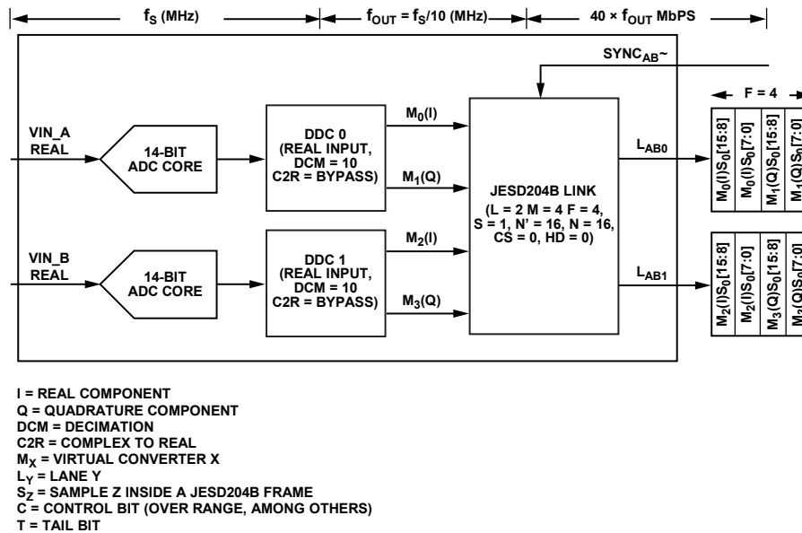
Figure 112. Two ADCs Plus Two DDCs Mode ( L = 2, M = 4, F = 4, S = 1 )
