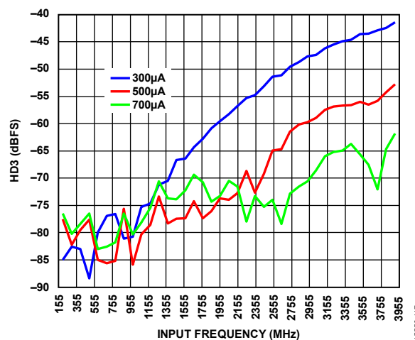
Figure 17. Third Harmonics ( HD3 ) vs. Input Frequency ( f_{IN} ) for Various Buffer Currents
