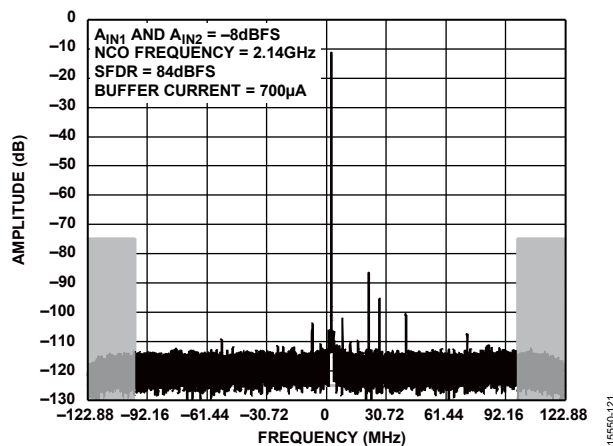
Figure 21. Two-Tone FFT; f_{IN1} = 1846.5 MHz, f_{IN2} = 2142.5 MHz f_{CLK} = 2.4576 GHz; Decimation Ratio = 10, NCO Frequency = 2140 MHz
