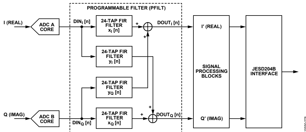
Figure 78. 24-Tap Full Complex Filter Configuration.
