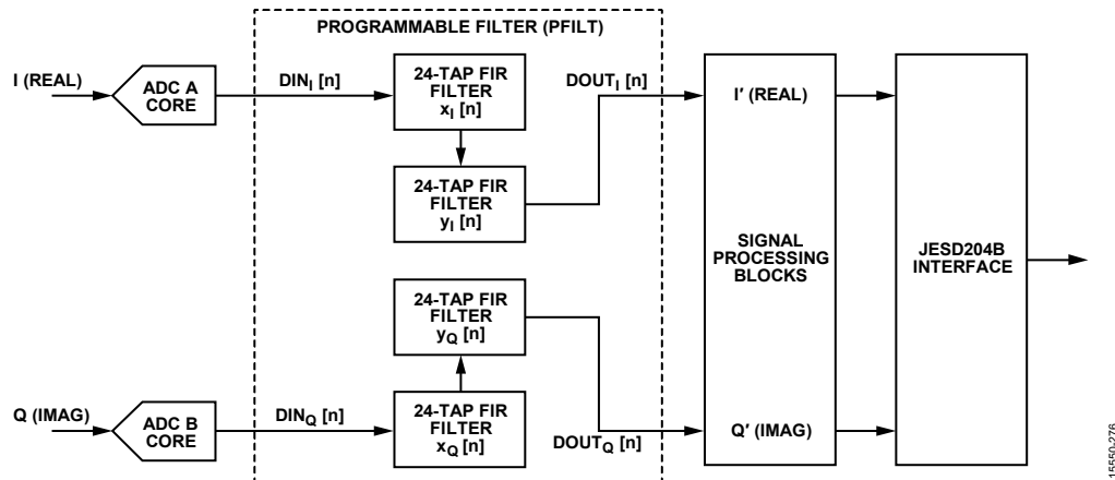
Figure 76. Real, Two Cascaded, 24-Tap Filter Configuration
