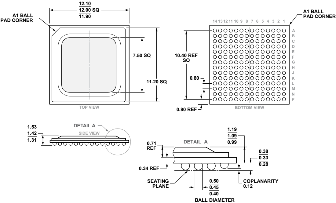
COMPLIANT TO JEDEC STANDARDS MO-275-GGAB-1. Figure 130. 196-Ball Ball Grid Array, Thermally Enhanced [BGA_ED] 12 mm x 12 mm (BP-196-4) Dimensions shown in millimeters
