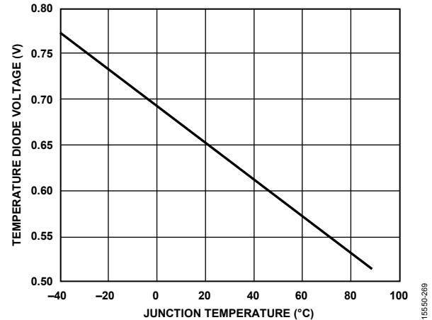
Figure 69. Typical Voltage Response of the 1× Temperature Diode
