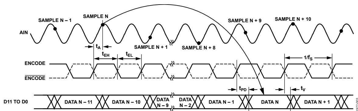
Figure 2. Timing Diagram
