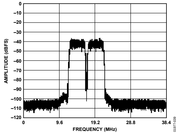
Figure 34. FFT: f_s = 76.8 MSPS, f_{IN} = 59.6 MHz, Two WCDMA Carriers, Differential AIN, SFDR Mode Enabled
