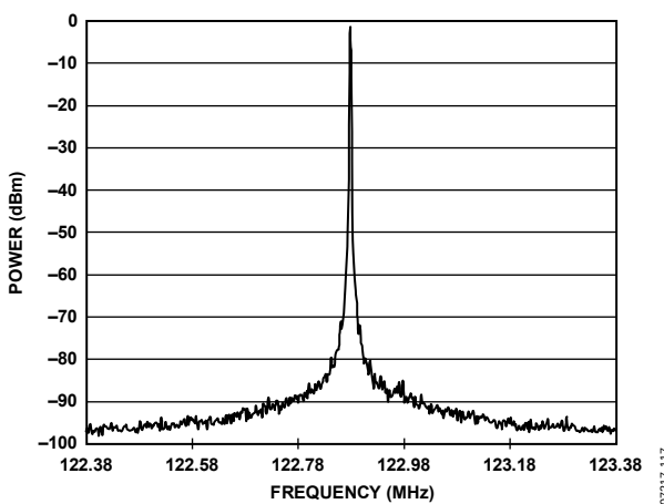
Figure 14. Output Spectrum, LVPECL; 122.88 MHz; PFD = 15.36 MHz; LBW = 127 kHz; I_{CP} = 3.0 mA; f_{VCO} = 1474.56 MHz
