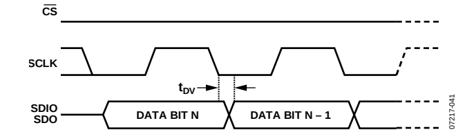
Figure 67. Timing Diagram for Serial Control Port Register Read
