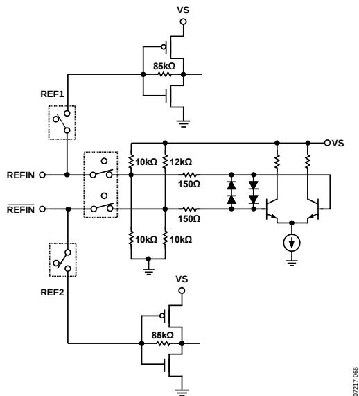
Figure 43. REF1N Equivalent Circuit for Non-XTAL Mode
