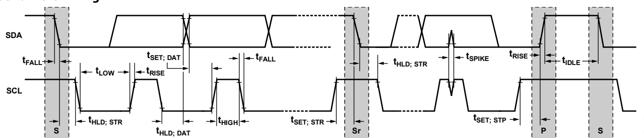
Figure 61. I 2 C Serial Port Timing
