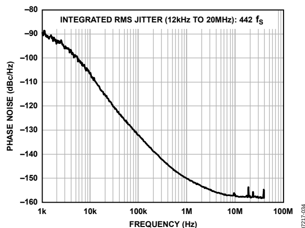
Figure 32. Phase Noise (Absolute) Clock Cleanup; Internal VCO at 1.552 GHz; PFD = 19.44 MHz; LBW = 1.84 kHz; LVPECL Output = 155.52 MHz
