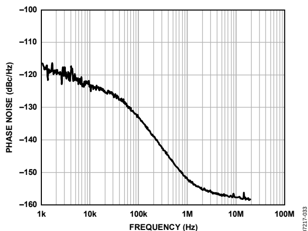
Figure 30. Phase Noise (Absolute) Clock Generation; Internal VCO at 1.475 GHz; PFD = 15.36 MHz; LBW = 40 kHz; LVPECL Output = 122.88 MHz
