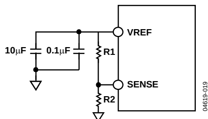
Figure 39. Programmable Reference
