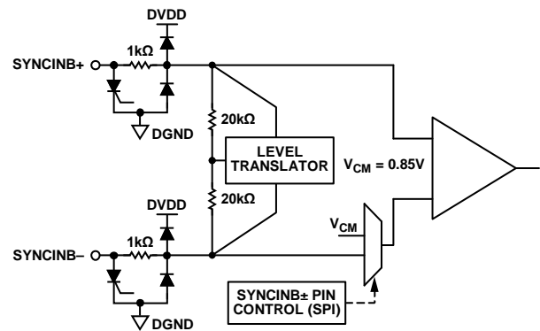
Figure 56. SYNCIN± Inputs
