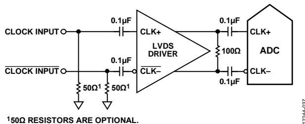
Figure 78. Differential LVDS Sample Clock
