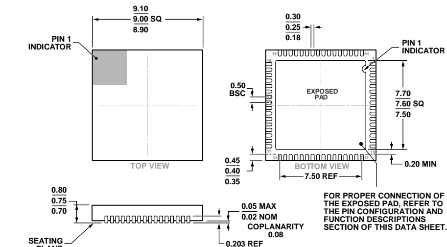
Figure 108. 64-Lead Lead Frame Chip Scale Package [LFCSP_WQ] 9 mm × 9 mm Body, Very Thin Quad (CP-64-15) Dimensions shown in millimeters
