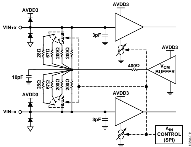
Figure 52. Analog Inputs
