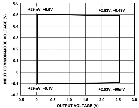
Figure 20. Input Common-Mode Voltage vs. Output Voltage, G = 100 , V_S = 2.7V , V_{REF} = 0V
