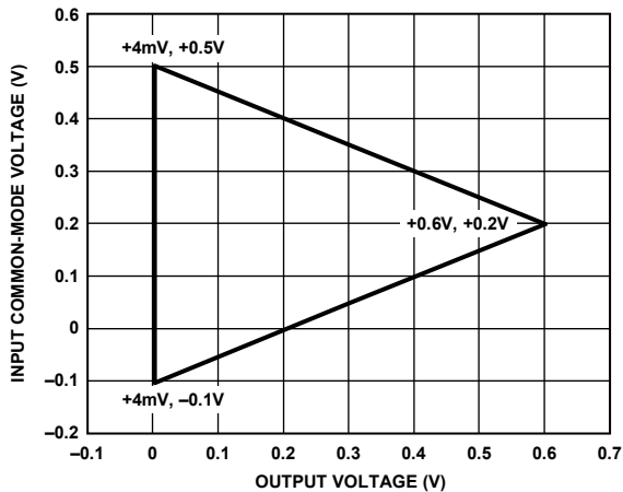
Figure 16. Input Common-Mode Voltage vs. Output Voltage, G = 1 , V_S = 2.7V , V_{REF} = 0V
