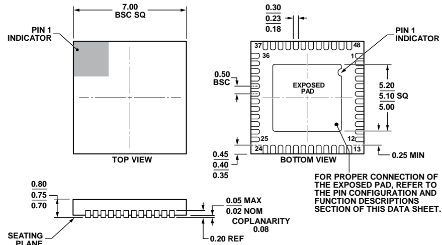
Figure 38. 48-Lead Lead Frame Chip Scale Package [LFCSP] 7 mm × 7 mm Body and 0.75 mm Package Height (CP-48-4)
