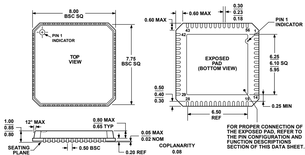
COMPLIANT TO JEDEC STANDARDS MO-220-VLLD-2 Figure 44. 56-Lead Lead Frame Chip Scale Package [LFCSP_VQ] 8 mm x 8 mm Body, Very Thin Quad (CP-56-1) Dimensions shown in millimeters
