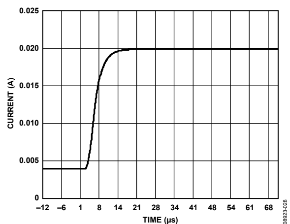
Figure 28. 4 mA to 20 mA Output Current Step
