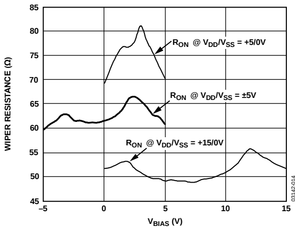
Figure 16. Wiper On-Resistance vs. Bias Voltage
