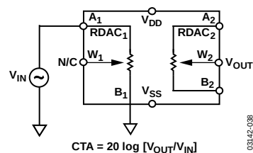
Figure 39. Test Circuit for Analog Crosstalk
