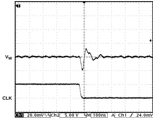
Figure 22. Digital Feedthrough
