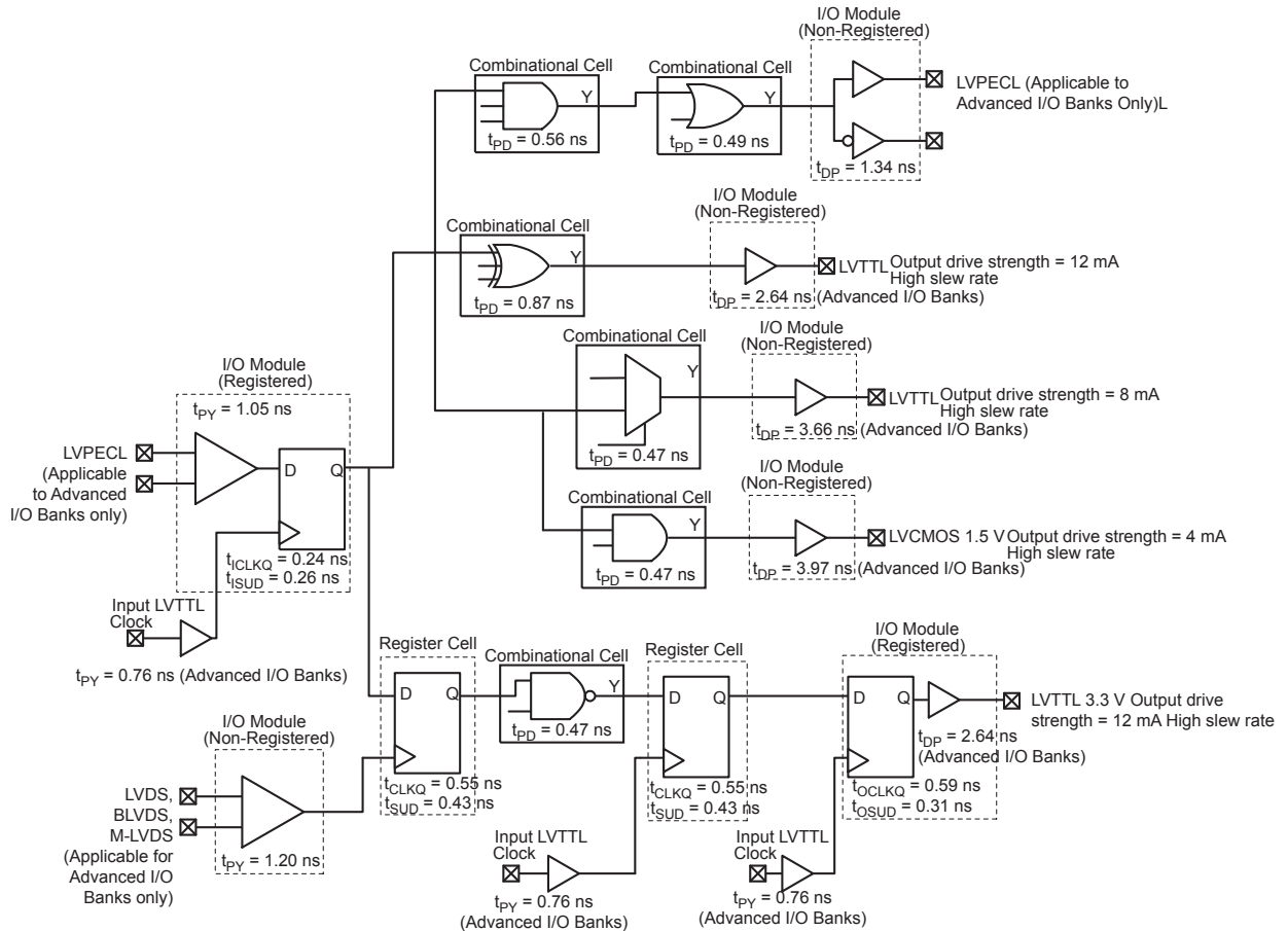
Figure 2-3 • Timing Model
