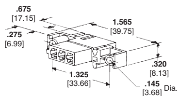
Receptacle Housing
