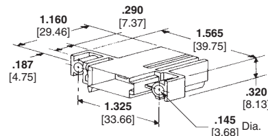
Tab Housing
