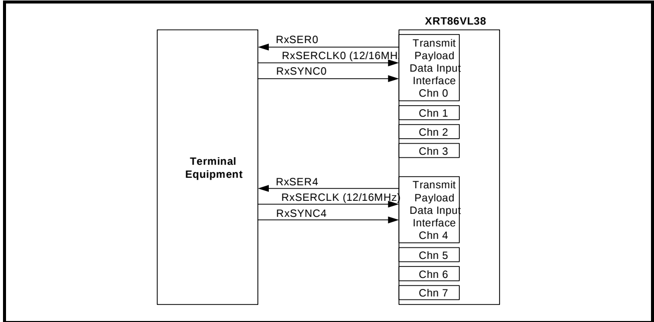
FIGURE 72. INTERFACING XRT86VL3X RECEIVE TO LOCAL TERMINAL EQUIPMENT USING 16.384Mbit/s, HMPV 16.384Mbit/s, AND H.100 16.384Mbit/s
