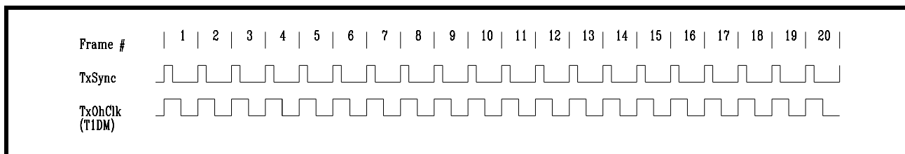
FIGURE 37. DS1 TRANSMIT OVERHEAD INPUT INTERFACE MODULE IN T1DM FRAMING FORMAT MODE
