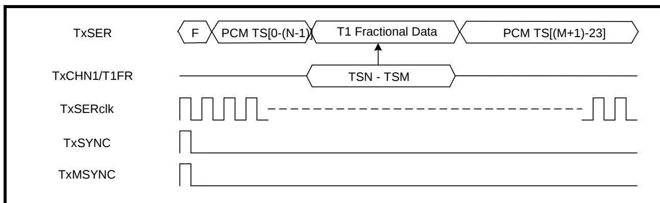
FIGURE 9. T1 FRACTIONAL INTERFACE
