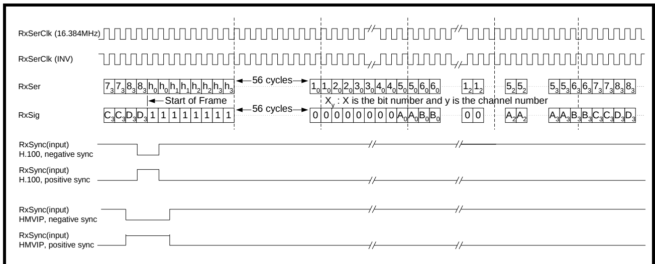
FIGURE 74. TIMING SIGNAL WEHN THE RECEIVE FRAMER IS RUNNING AT HMPV AND H100 16.384MHz MODE
