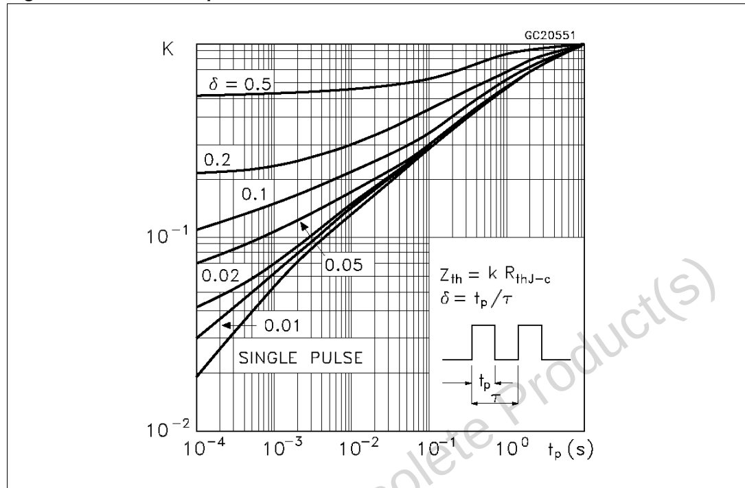
Figure 8. Thermal impedance for ISOWATT220
