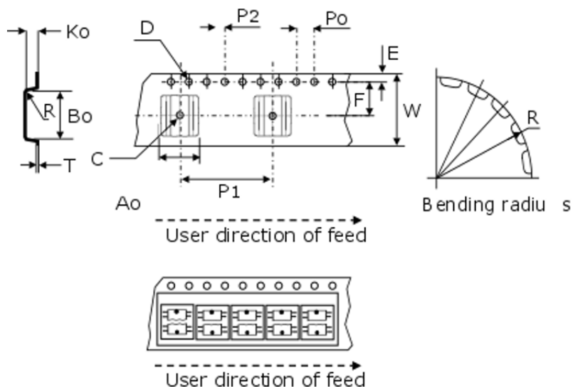
Figure 20. Tape specifications
