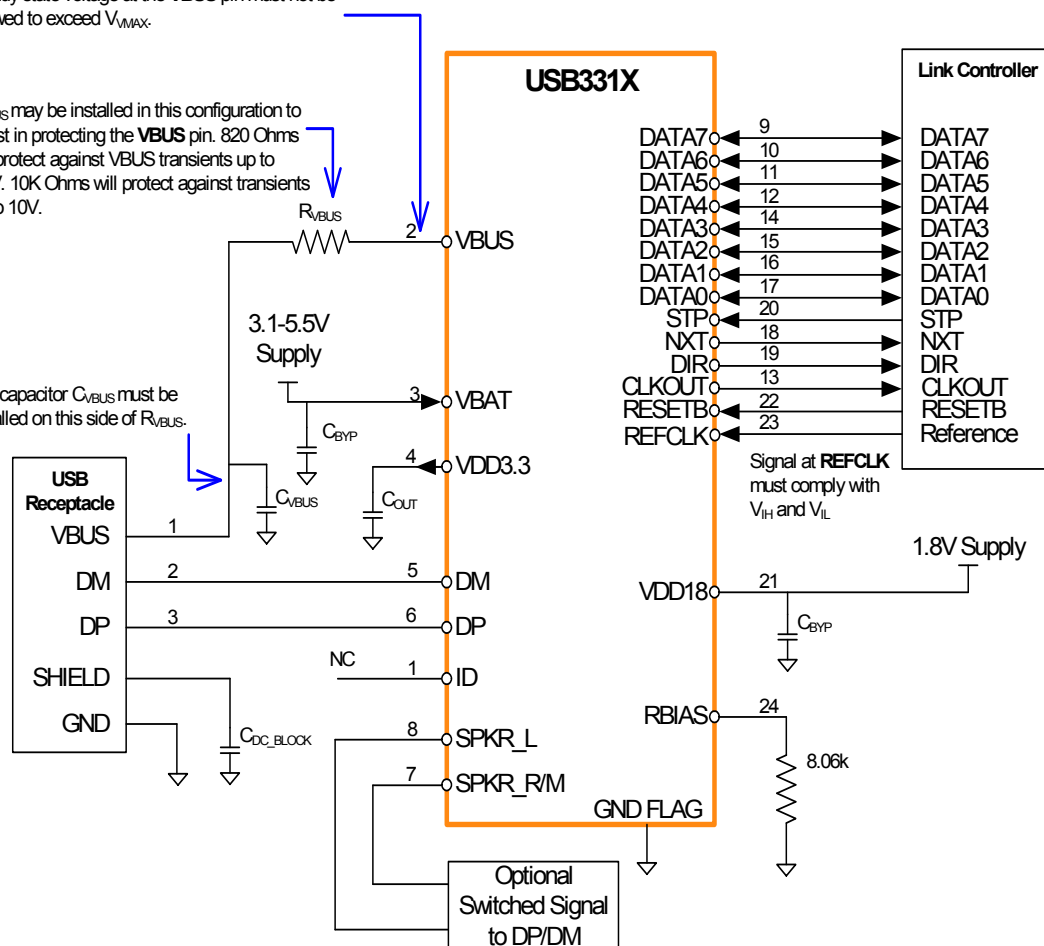
Figure 8.1 USB3311 QFN Application Diagram (Device)
