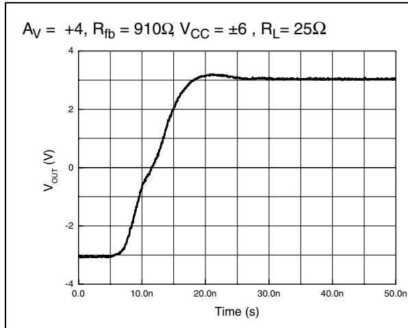
Figure 12. Positive slew rate
