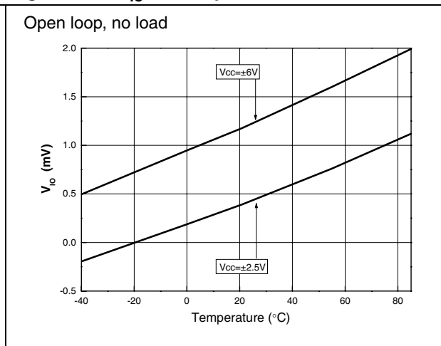
Figure 39. V_{io} vs. temperature
