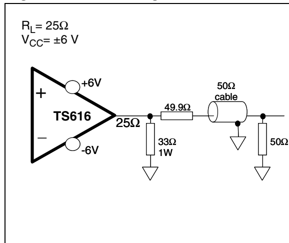
Figure 2. Load configuration
