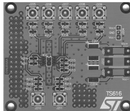
Figure 56. Evaluation board
