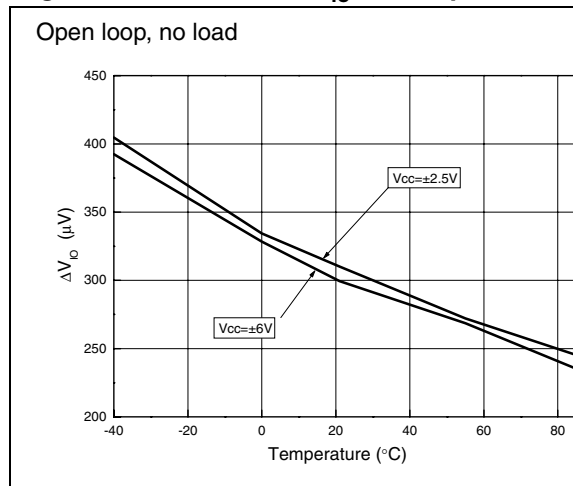
Figure 38. Differential V_{io} vs. temperature
