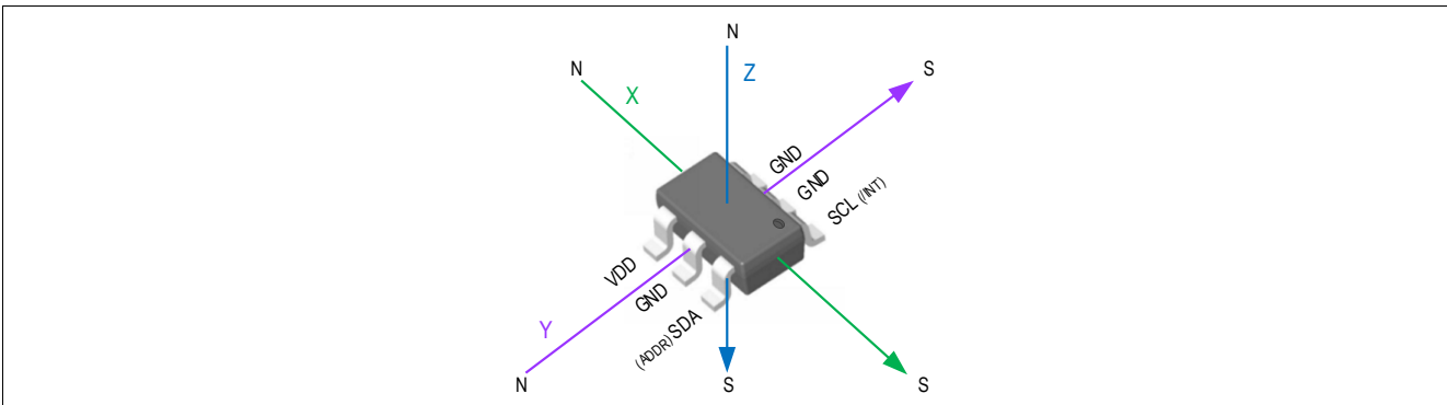
Figure 1 All three Sensitive Directions Bx, By and Bz
