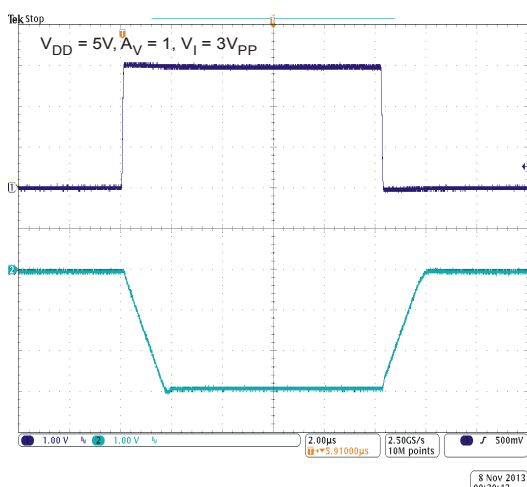
Figure 24 Inverting Large Signal Pulse Response V_{DD} = 5V
