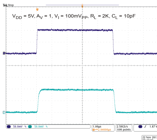
Figure 23 Voltage Follower Small Signal Pulse Response
