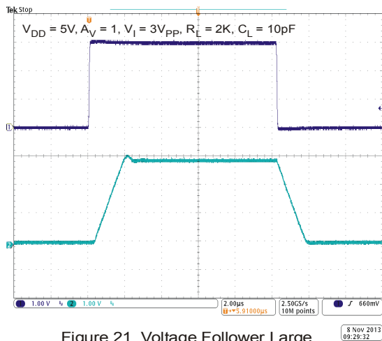
Figure 21 Voltage Follower Large Signal Pulse Response V_{DD} = 5V
