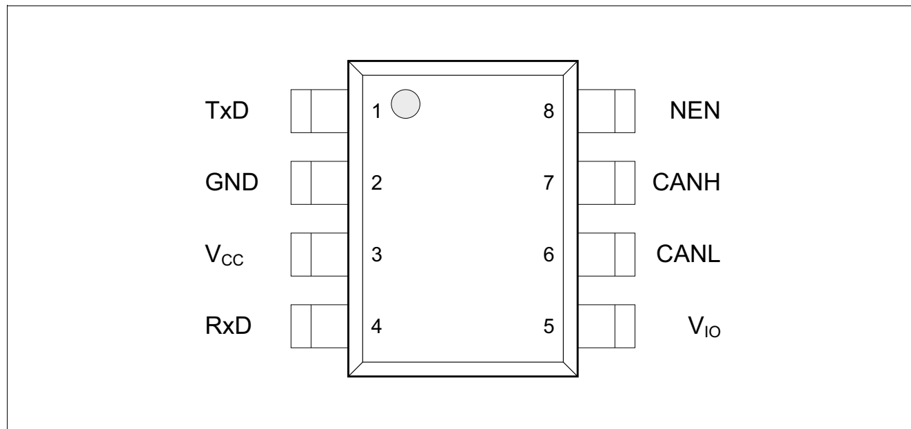
Figure 2 Pin configuration
