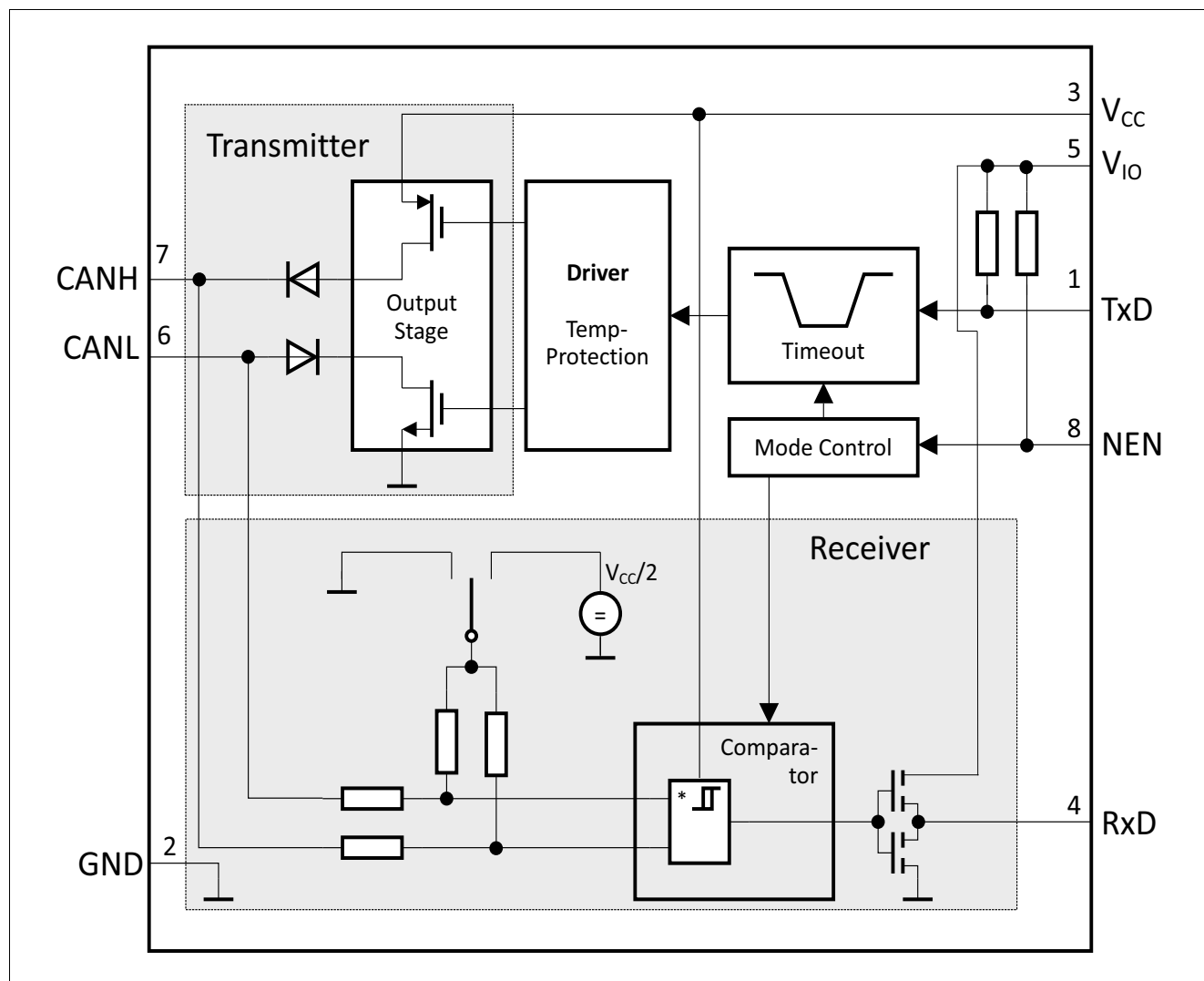
Figure 1 Block diagram
