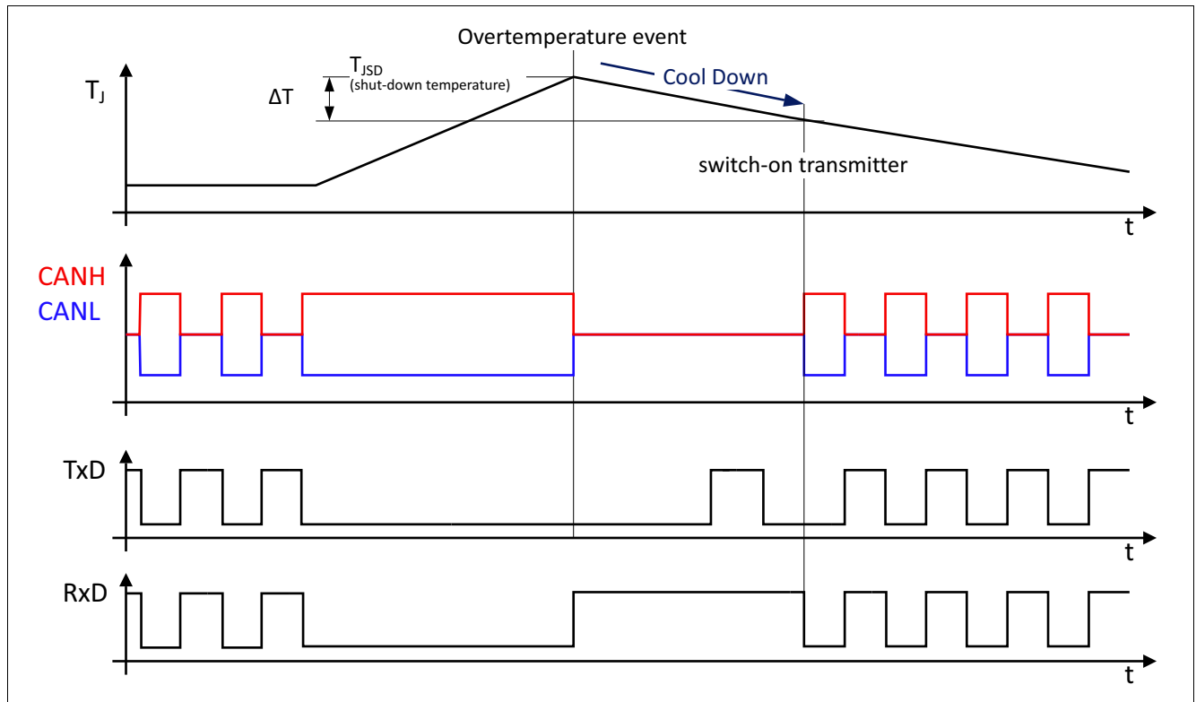
Figure 7 Overtemperature protection
