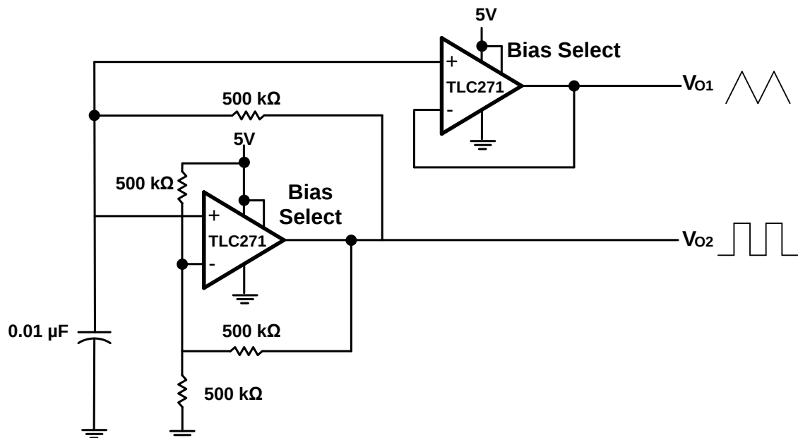
Figure 110 Multivibrator
