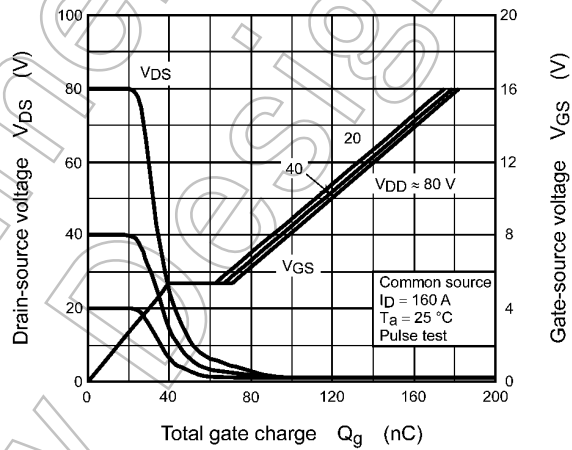
Fig. 9.10 Dynamic Input/Output Characteristics
