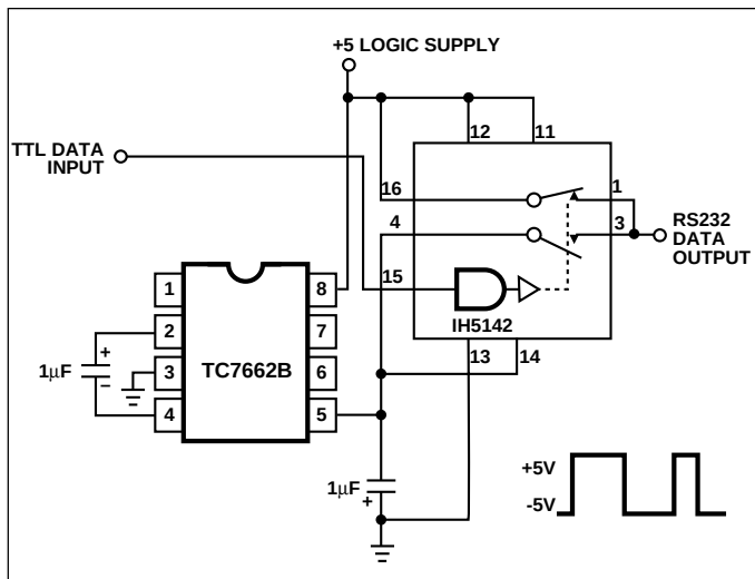
Figure 13. RS232 Levels from a Single 5V Supply
