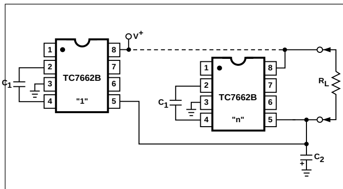
Figure 5. Paralleling Devices
