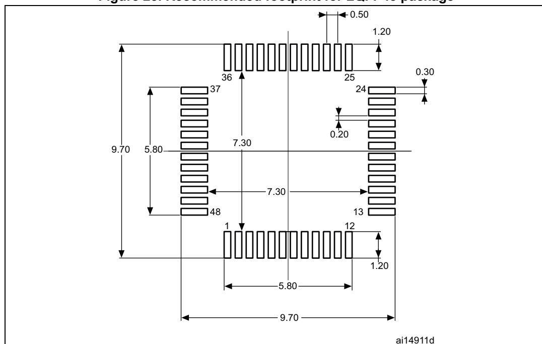
Figure 28. Recommended footprint for LQFP48 package
