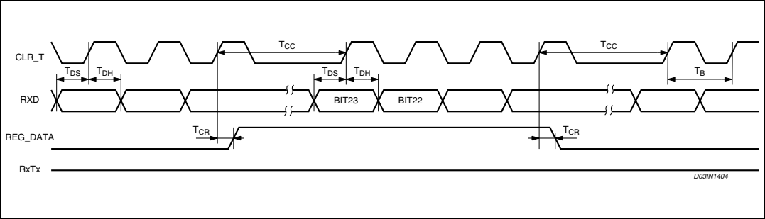
Figure 6. Data reception -> control register read -> data reception timing diagram
