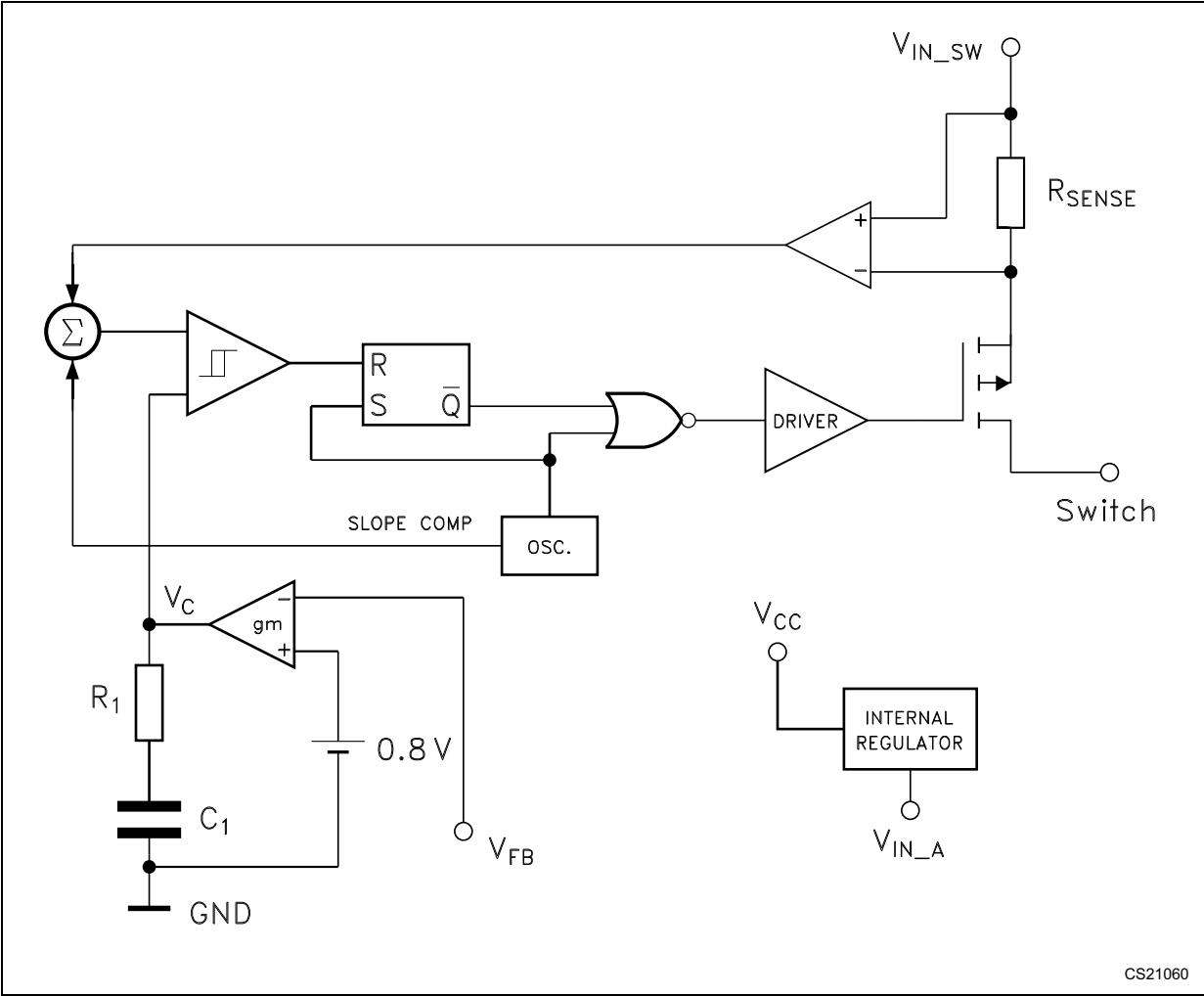
Figure 1. Schematic diagram
