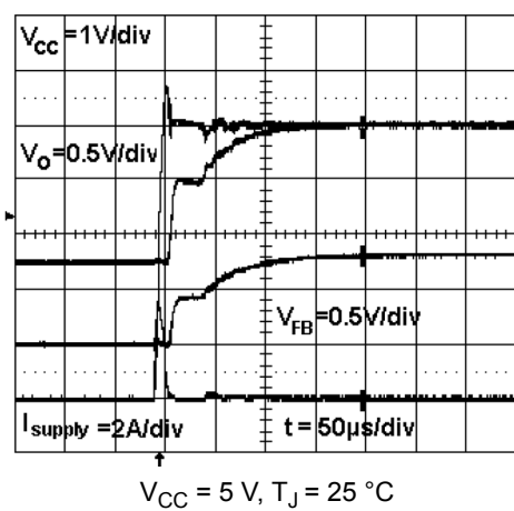
Figure 21. Startup transient
