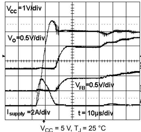
Figure 20. Startup transient
