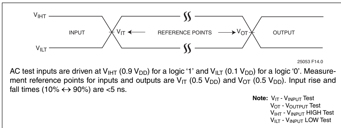
Figure 20: AC Input/Output Reference Waveforms
