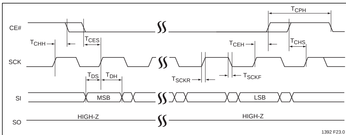
Figure 23: Serial Input Timing Diagram
