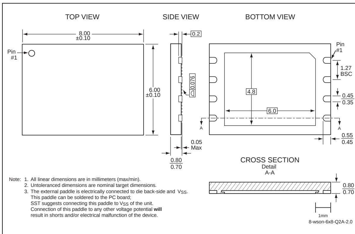
Figure 30: 8-Contact Very-very-thin Small Outline No-lead (WSN) SST Package Code: Q2A
