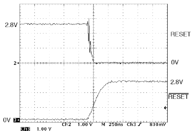
Figure 13: SP708 RESET and RESET De-Assertion
