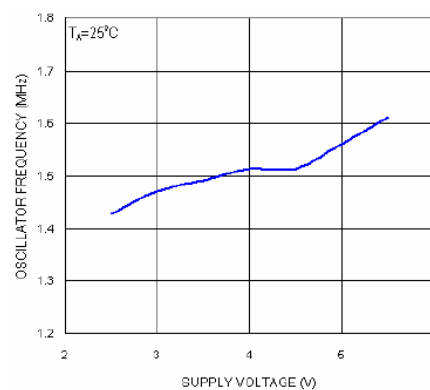
Fig. 15: Oscillator Frequency vs Supply Voltage
