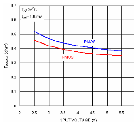
Fig. 11: R_{DS(ON)} vs Input Voltage
