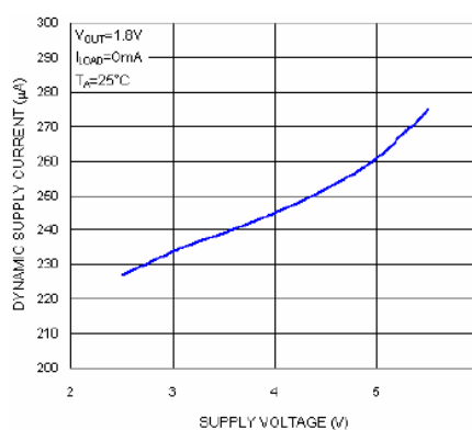
Fig. 13: Dynamic Supply Current vs Supply Voltage
