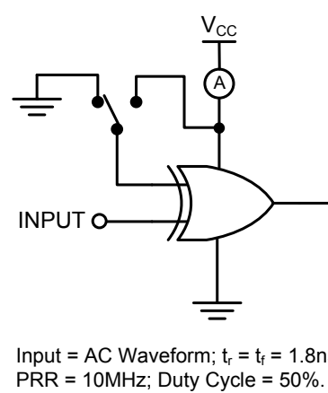
Figure 3. ICCD Test Circuit
