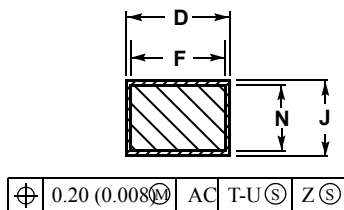
SECTION AE-AE
