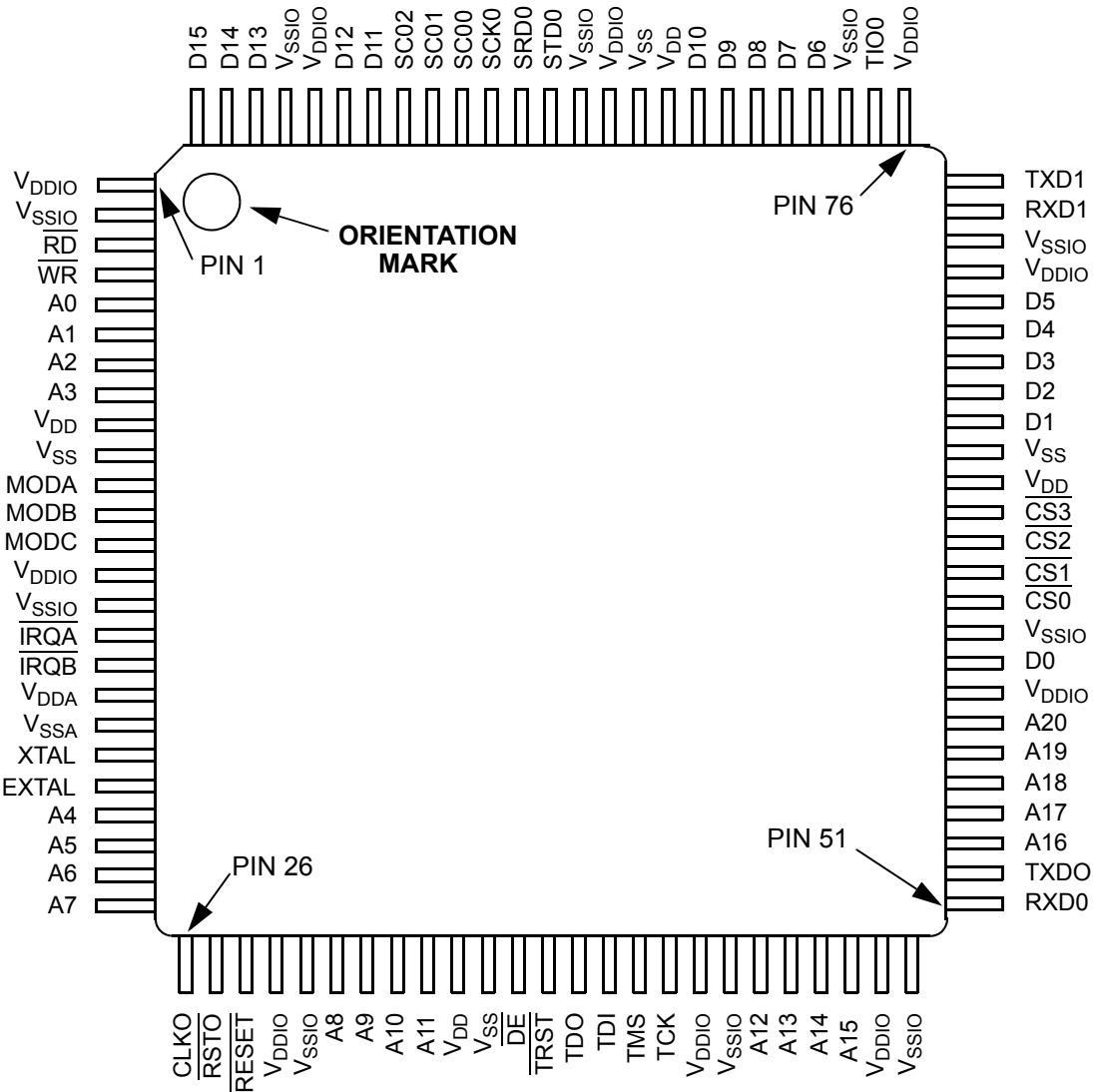
Figure 5-1 Top View, 56855 100-pin LQFP Package
