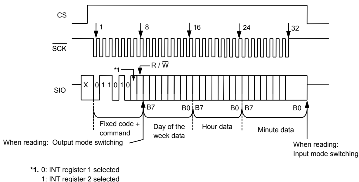
Figure 38 INT Register 1 Access and INT Register 2 Access
