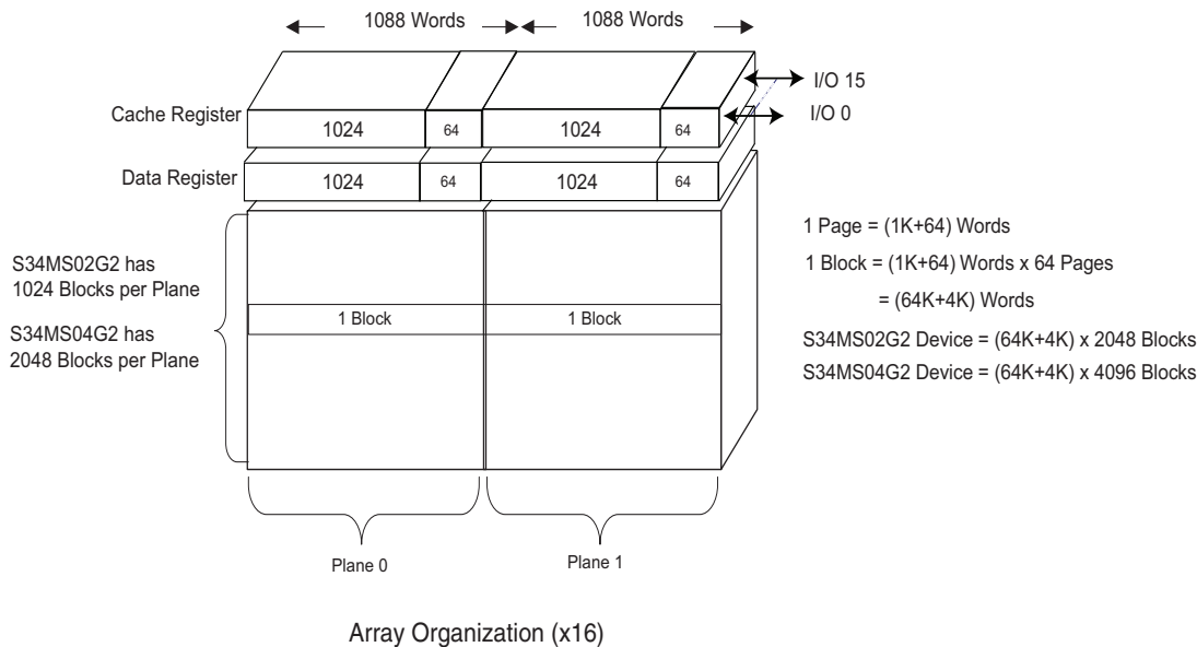
Figure 1.10 Array Organization — S34MS02G2 and S34MS04G2 (x16)
