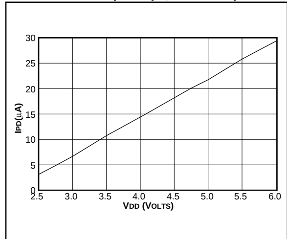
FIGURE 18-13: MAXIMUM I_{PD} vs. TIMER1 ENABLED (32 kHz, RC0/RC1 = 33 \text{ pF}/33 pF, 85^{\circ}\text{C TO } -40^{\circ}\text{C} , RC MODE)
