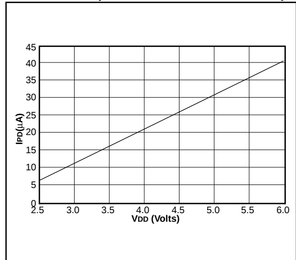
FIGURE 18-13: MAXIMUM I_{PD} vs. TIMER1 ENABLED (32 kHz, RC0/RC1 = 33 \text{ pF}/33 pF, 85^{\circ}\text{C TO } -40^{\circ}\text{C} , RC MODE)
