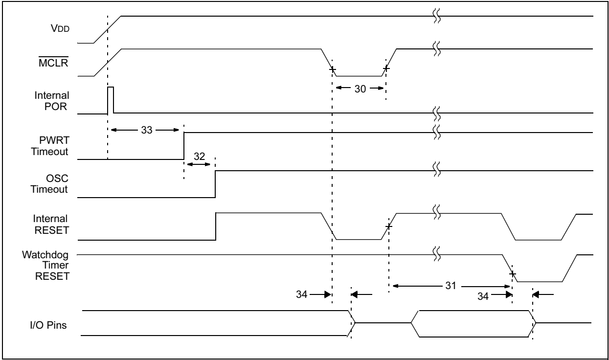
FIGURE 17-8: RESET, WATCHDOG TIMER, OSCILLATOR START-UP TIMER AND POWER-UP TIMER TIMING
