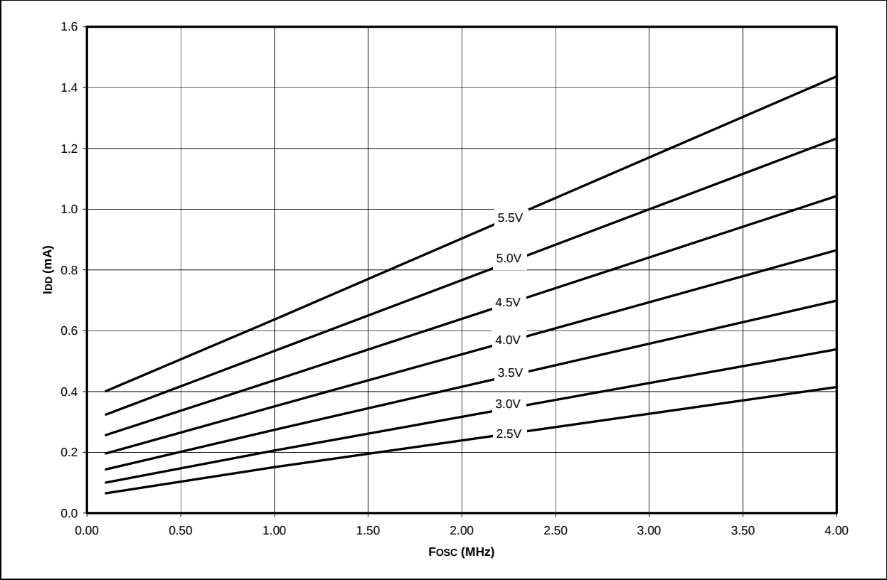
FIGURE 16-3: MAXIMUM I_{DD} VS. F_{osc} OVER V_{DD} (XT MODE)
