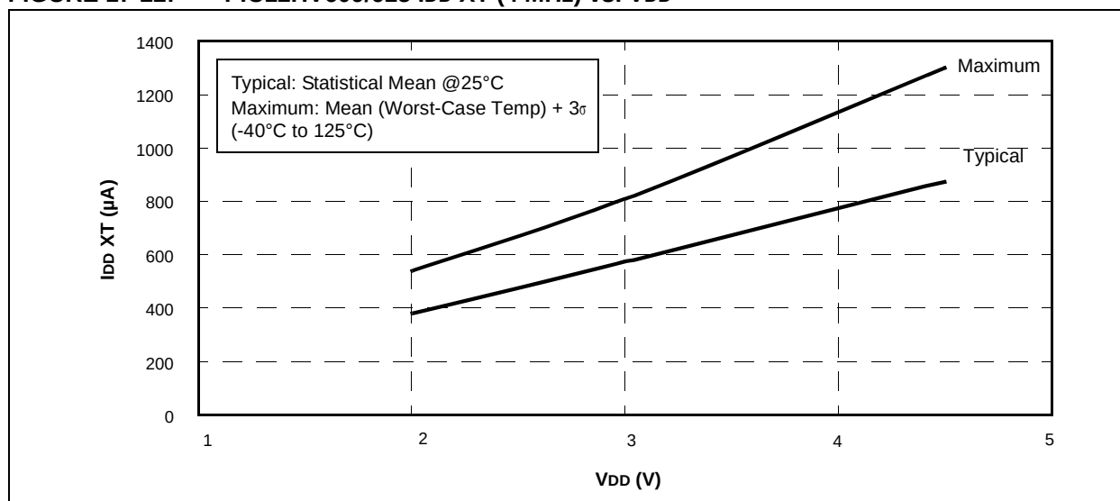
FIGURE 17-22: PIC12HV609/615 I_{DD XT} (4 MHz) vs. V_{DD}
