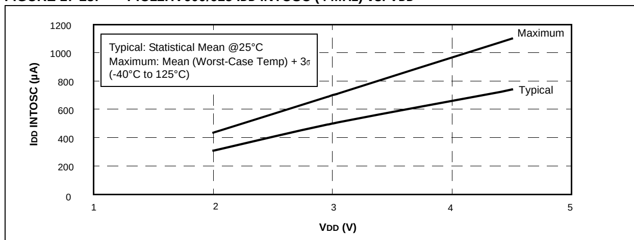
FIGURE 17-23: PIC12HV609/615 I_{DD INTOSC} (4 MHz) vs. V_{DD}
