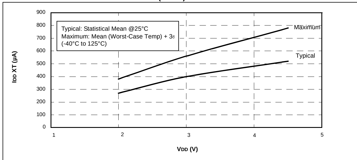
FIGURE 17-21: PIC12HV609/615 I_{DD XT} (1 MHz) vs. V_{DD}
