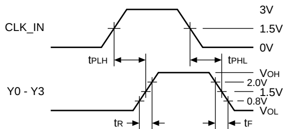
Propagation Delay
