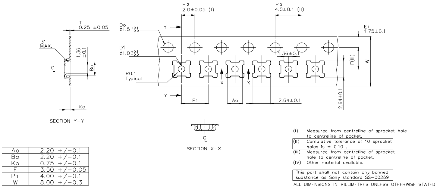
Figure 23. Tape and Reel Specifications
