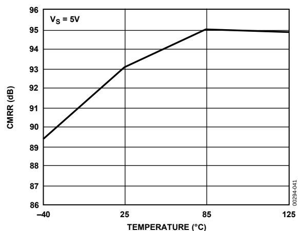
Figure 36. CMRR vs. Temperature, V_S = 5V
