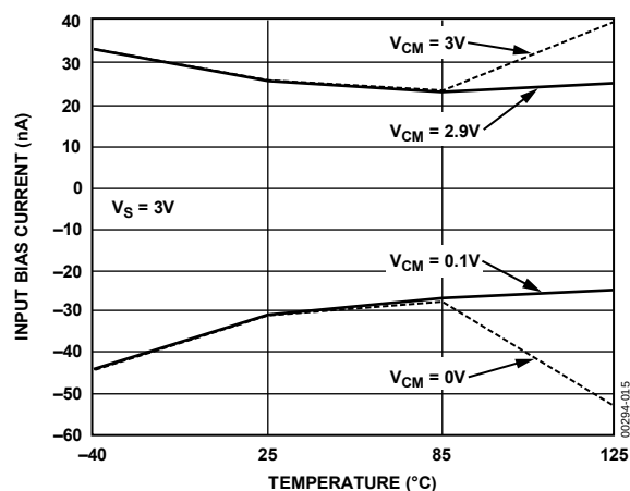
Figure 10. Input Bias Current vs. Temperature, V_S = 3V
