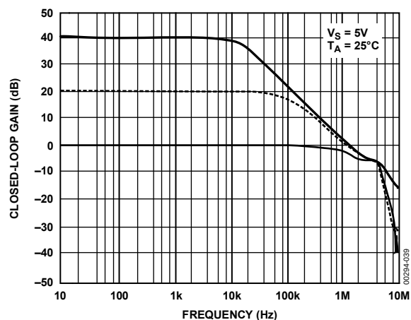
Figure 34. Closed-Loop Gain vs. Frequency, V_S = 5V
