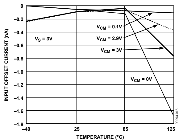
Figure 11. Input Offset Current vs. Temperature, V_S = 3V
