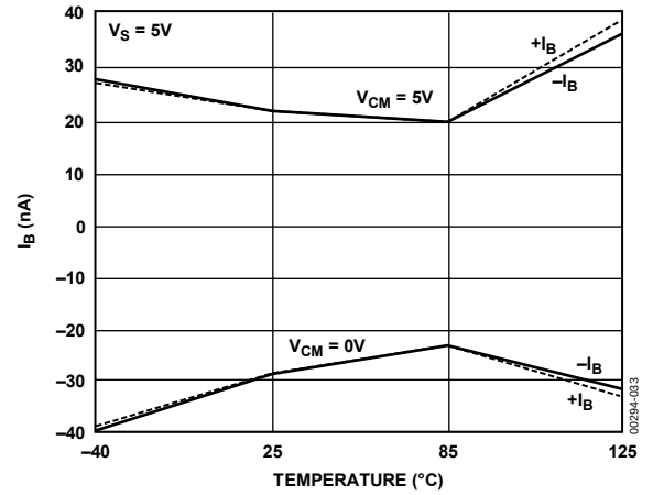
Figure 28. Input Bias Current vs. Temperature, V_S = 5\text{ V}
