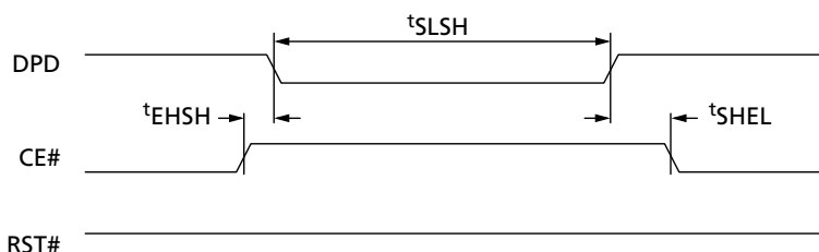
Figure 18: Deep Power-Down Operation Timing
