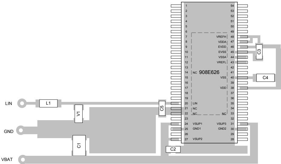
Figure 19. PCB Layout Recommendations
