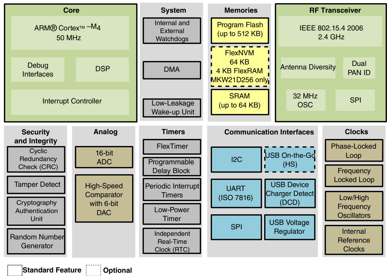
Figure 1. MKW2xD simplified block diagram
