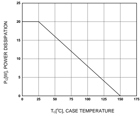
Figure 1. Power Derating
