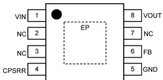
8-Pin ePAD MSOP MIC5282YMME (TOP VIEW)
