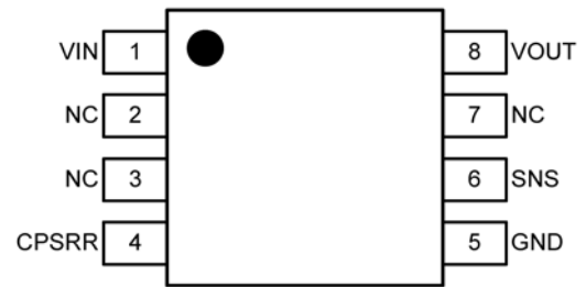
8-Pin MSOP MIC5282-x.xYMM (TOP VIEW)
