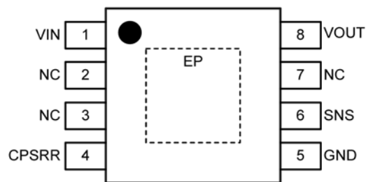
8-Pin ePAD MSOP MIC5282-x.xYMME (TOP VIEW)
