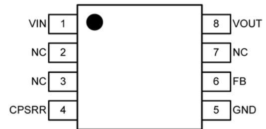
8-Pin MSOP MIC5282YMM (TOP VIEW)
