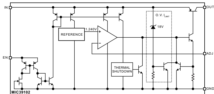
MIC39102 Adjustable Regulator
