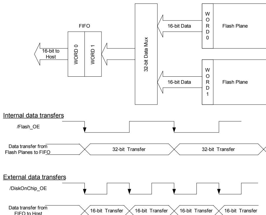
Figure 15: MultiBurst Operation
