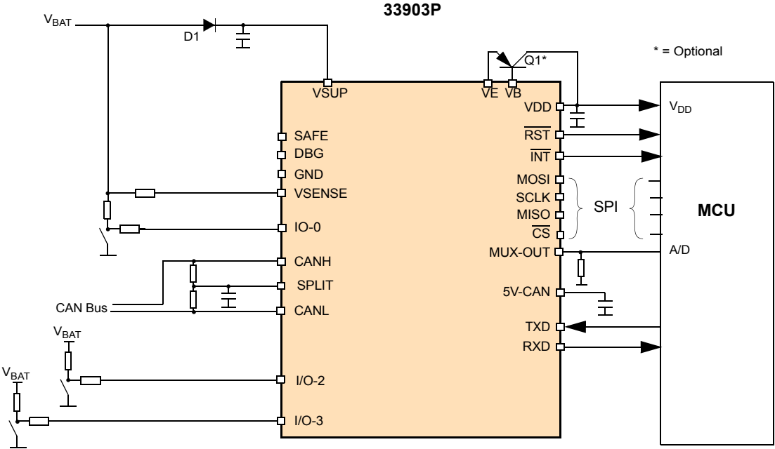
Figure 7. 33903P simplified application diagram
