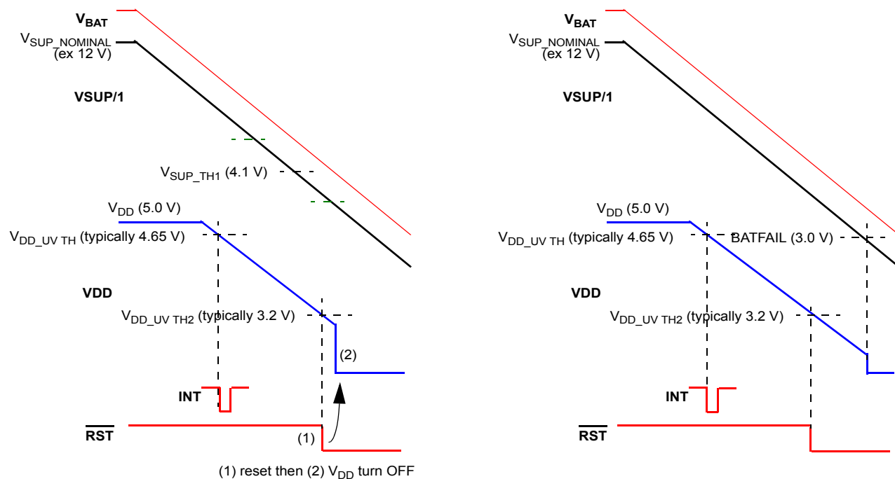
Case 6: "V DD UV 3.2V", with bit Crank = 1
