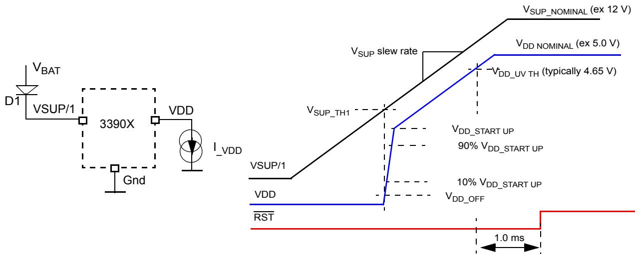
Figure 28. V_{DD} start-up versus V_{SUP/I1} ramp
